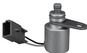
T76425 AODE MCCC Fits 92- Early 95 AODE 1-3 Ohms, OEM Plug Compatible
