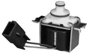
T86420 AXODE/ AX4S/ AX4N SHIFT Fits 91-94 AXODE, 95-04 AX4S, 95-07 AX4N 15-25 Ohms, OEM Plug Compatible
