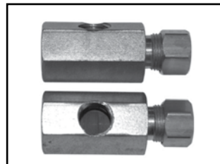
CR-1008 Three Way Fitting for making parallel coolers with one line to the transmission and one each to the radiator cooler and the external cooler.
