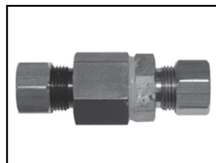
CR-1012 5/16" Compression Union with One Way Valve CR-1014 3/8" Compression Union with One Way Valve CR-1016 1/2" Compression Union with One Way Valve
